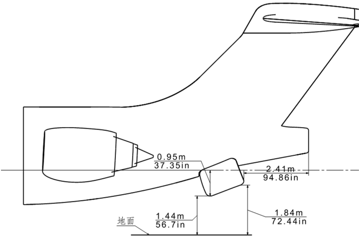
ICN-ARJ21-A-192002-A-SVV19-10752-A-001-01
